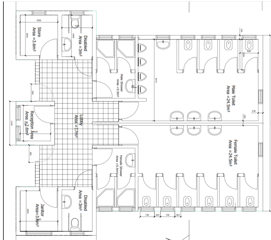
Figure 6: Floor Plan for Public Toilet
